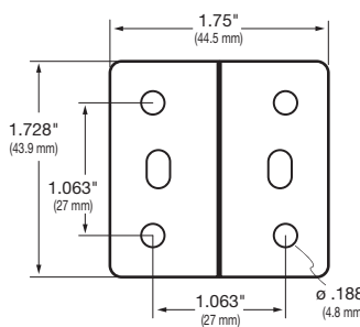
Keyboard/Laptop Pivot Interface
