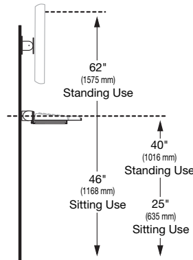
100 Series (Fixed Height)
